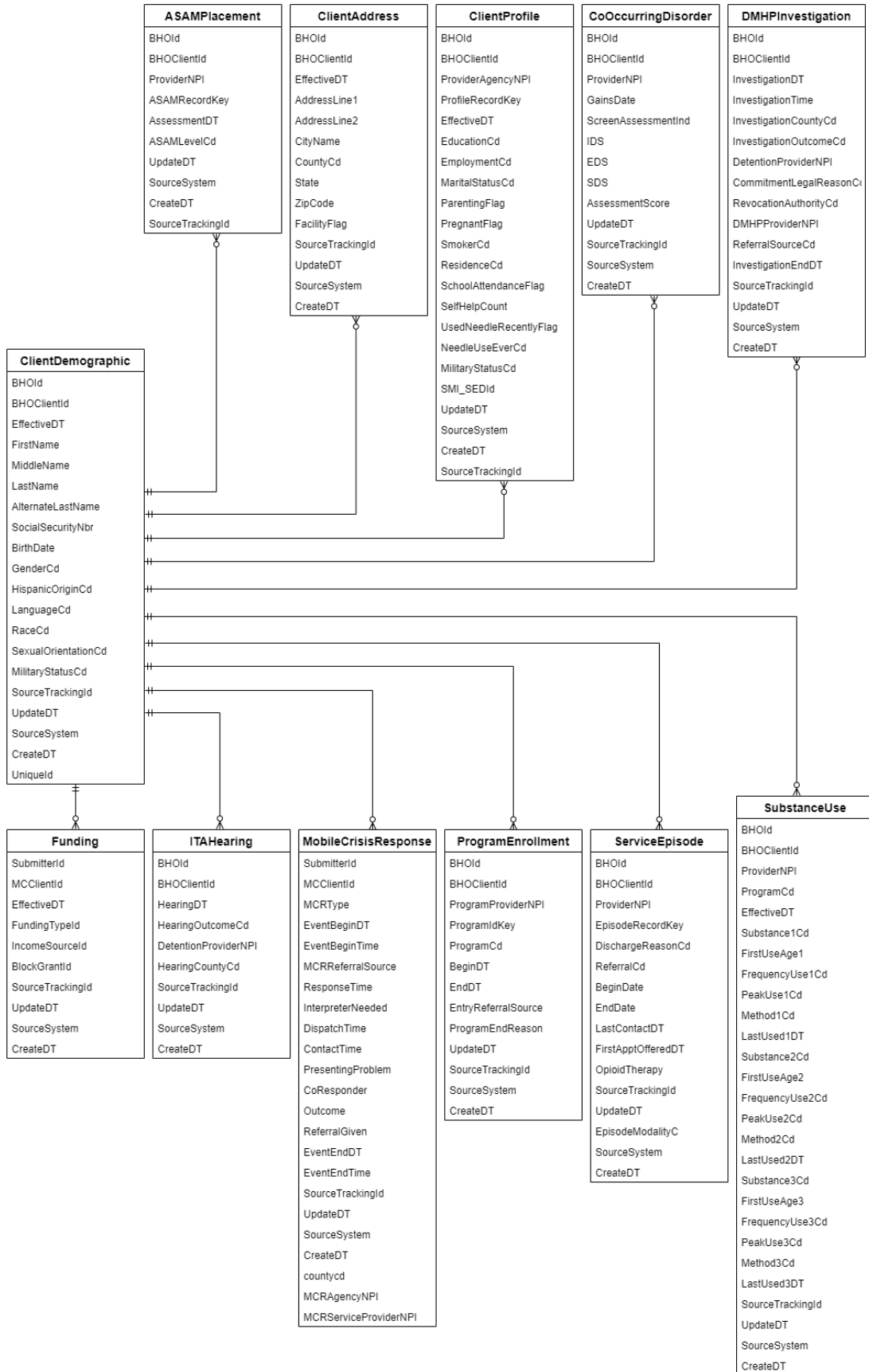
Appendix C: Entity Relationship Diagram (ERD) Excerpt from Behavioral Health Data Guide v5.7
