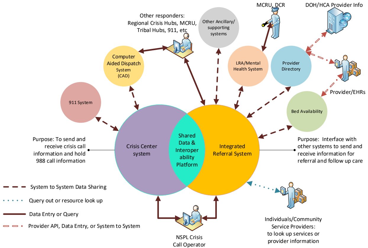
Figure 4 Data Flow
